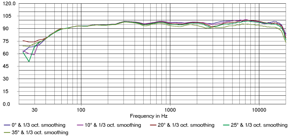
W2 Horizontal Magnitude in dB SPL/2.83V at 1 meter
