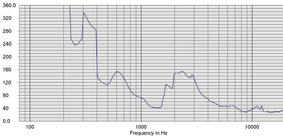
W2 Vertical Beamwidth
