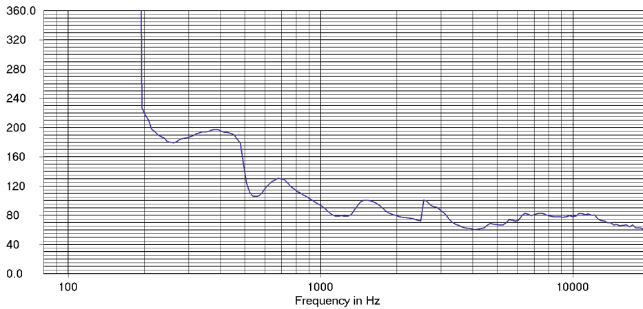
W2 Horizontal Beamwidth
