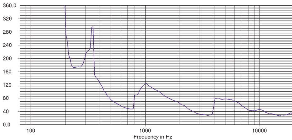
W3 Vertical Beamwidth
