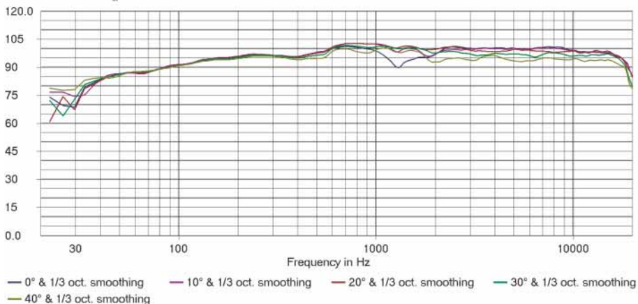
AMI2 Horizontal Magnitude in dB SPL/2.83V at 1 meter
