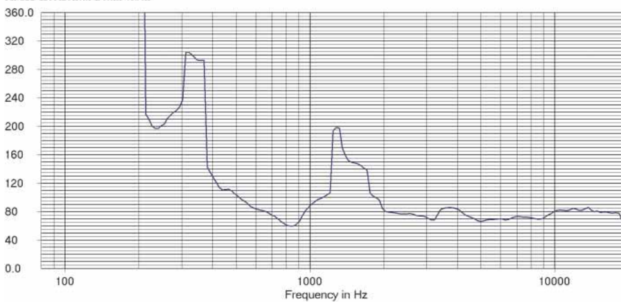
AMI2 Vertical Beamwidth
