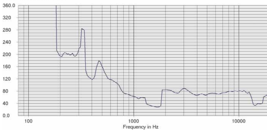
AM15 Vertical Beamwidth
