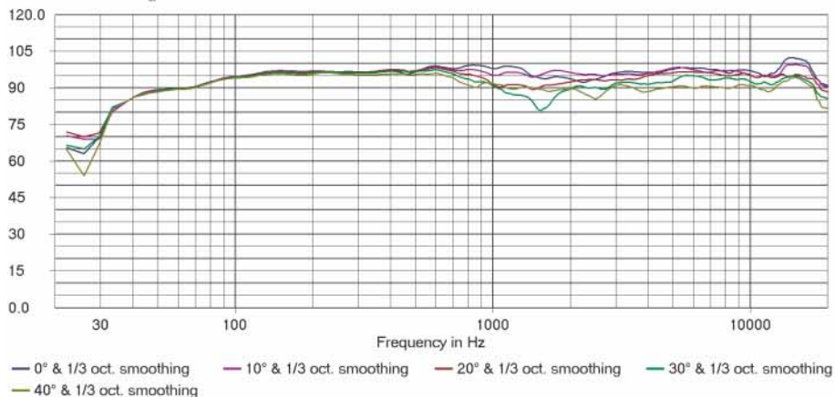
AM15 Horizontal Magnitude in dB SPL/2.83V at 1 meter
