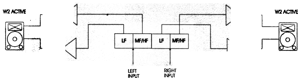
FIG. 4 W2 Active Configuration using WX3AW2LF card
