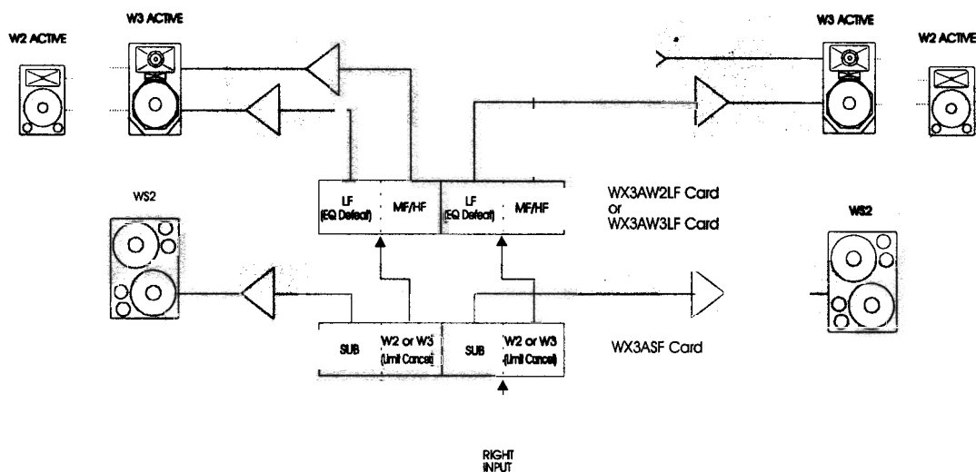
FIG. 9 Normal Operation for augmenting stereo W2 Active/W3 with Sub Bass
